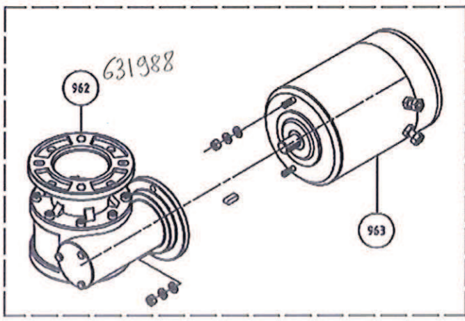
CLIPPER 1300
